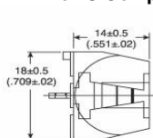
PCB/Mounting Layout
