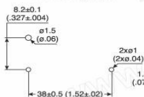
PCB/Mounting Layout
